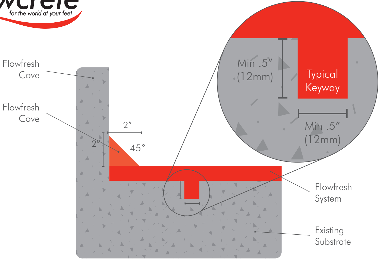
Typical 2" Cant Cove
